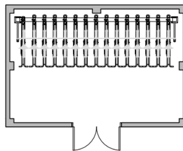
CYCLE STORE PLAN
