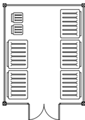
BIN STORE PLAN
